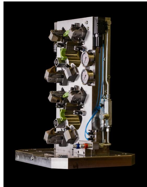
2. Fixtures for CNC machining
