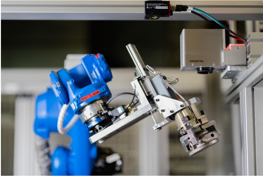
ROBOTIC LASER ENGRAVING OF DMC.
