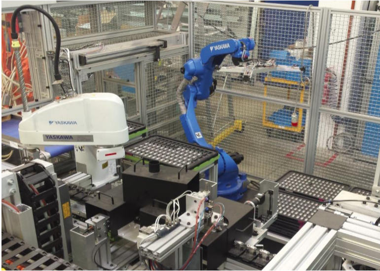
ROBOTIC PACKAGING UNITS
