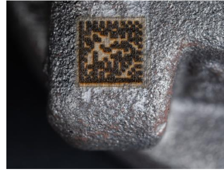
DATA MATRIX CODE ON Fe CASTING
